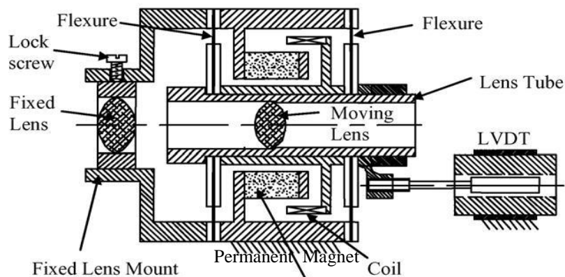
Fig 2. Schematic of programmable focusing mechanism.
