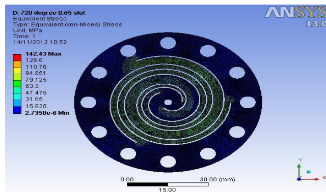
Fig 14. Flexure bearing with 720° spiral and 0.65mm slot thickness
