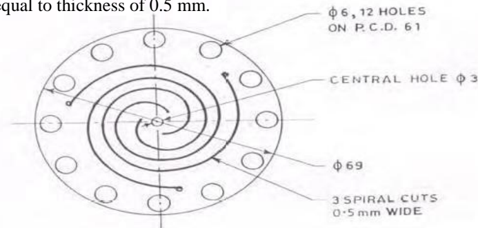
Fig 4 Typical Flexural Unit For Linear Compressor bearing
