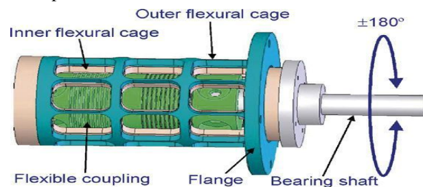
Figure 1 Schematic view of the bearing as a \mu -spindle.
