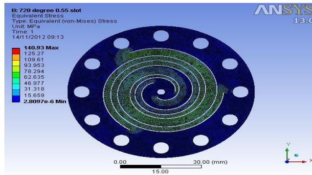
Fig 12. Flexure bearing with 720° spiral and 0.55mm slot thickness
