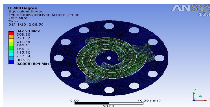
Fig 8. Flexure bearing with 480° spiral
