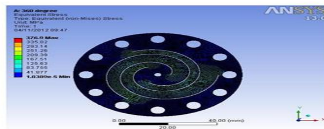
Figure 7 Flexure bearing with 360° spiral
