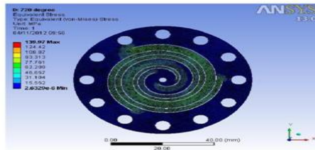
Fig 10. Flexure bearing with 720° spiral
