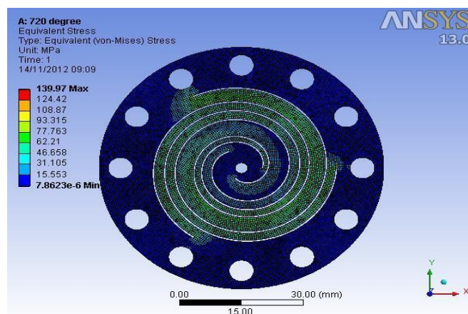
Fig 11. Flexure bearing with 720° spiral and 0.5mm slot thickness
