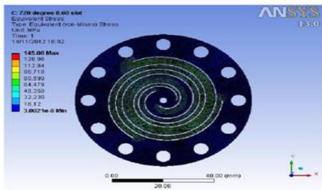
Fig 13. Flexure bearing with 720° spiral and 0.60mm slot thickness
