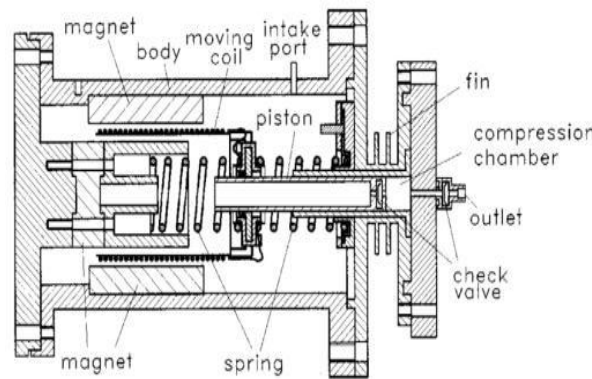
Fig 3. Schematic of Linear Compressor
