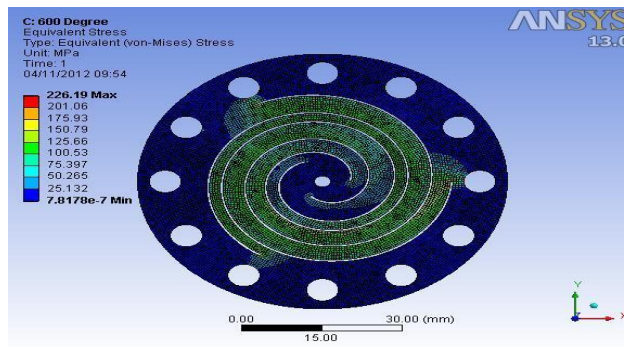
Fig 9. Flexure bearing with 600° spiral
