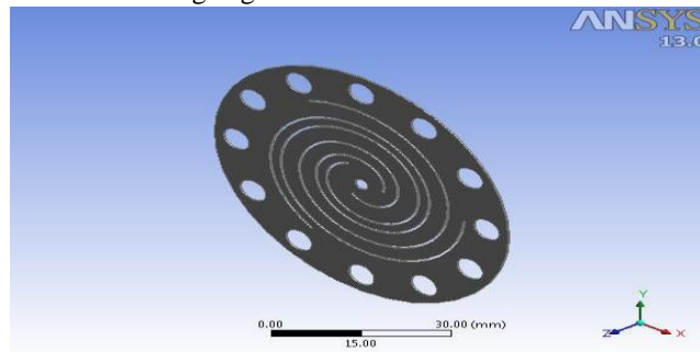
Fig 6. Ansys Model For Flexure Bearing
